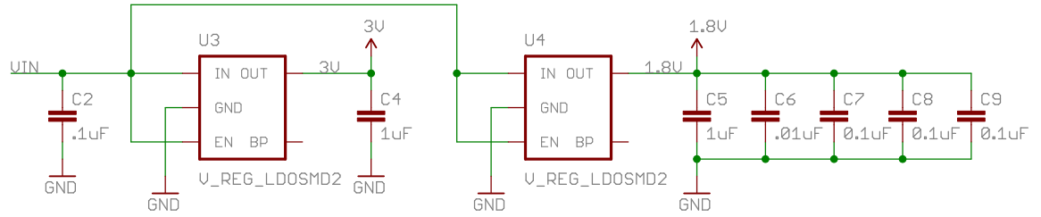
Power Section
