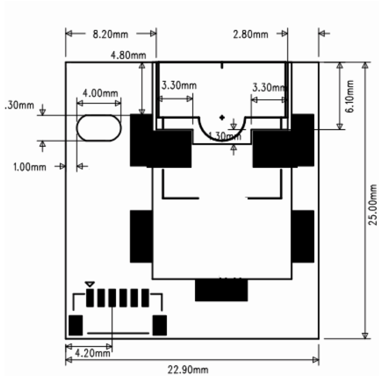
Figure 1: Board dimension
