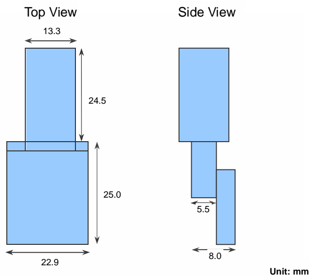
Figure 2: Main board with active antenna dimension
