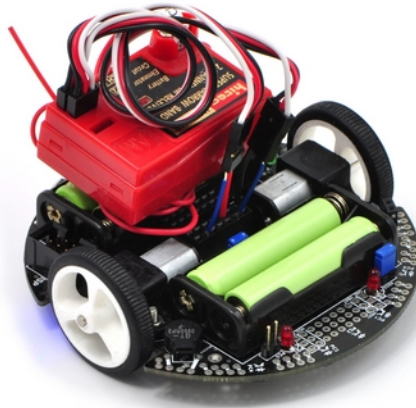
A radio-controlled 3pi.
