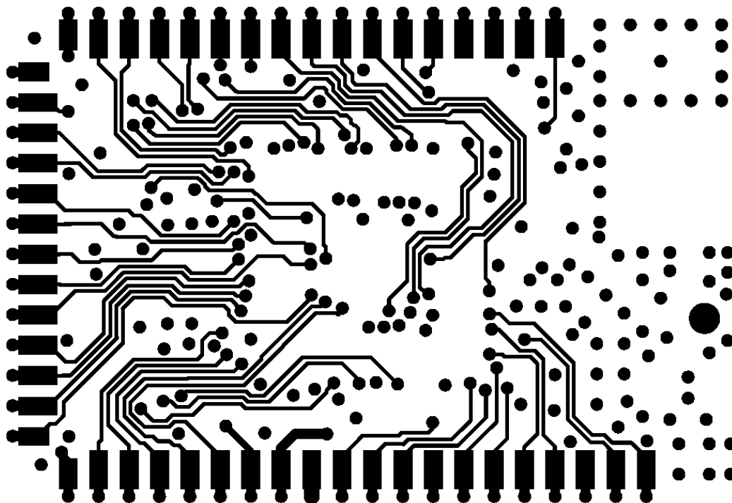
Figure 40: Bottom side layout of the module. Any via in the module can cause a short if placed directly above bare copper on a PCB.
