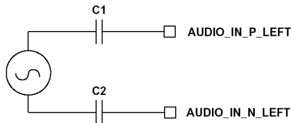
Figure 19: Differential input (left channel shown)
