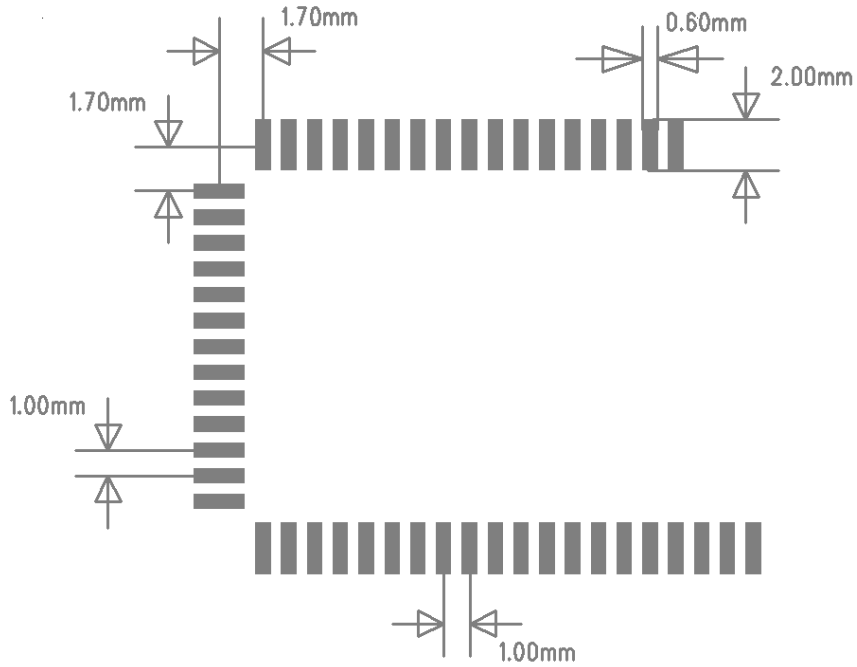
Figure 41: Recommended PCB land pattern
